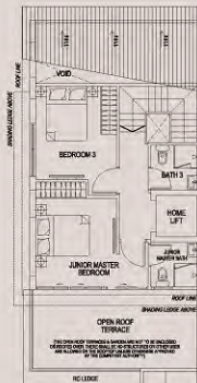
ATTIC PLAN
