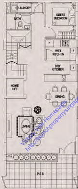
1ST STOREY PLAN
