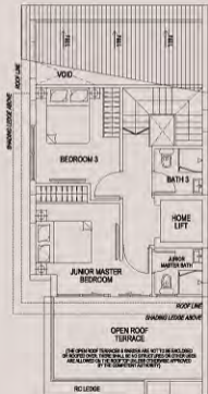
ATTIC PLAN
