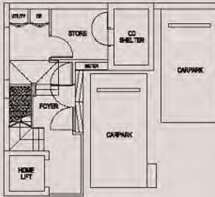
BASEMENT PLAN
