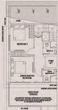
ATTIC PLAN
